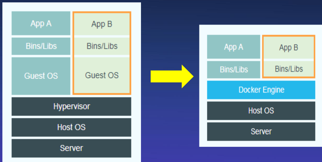
Virtual Machine
