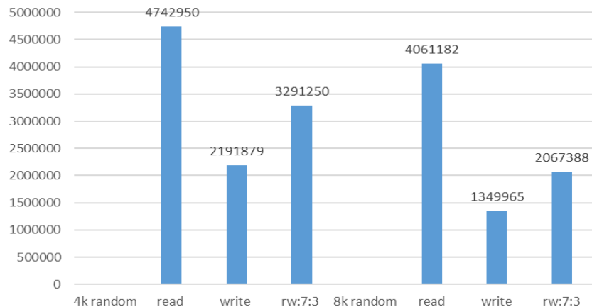
24 volumes iops
