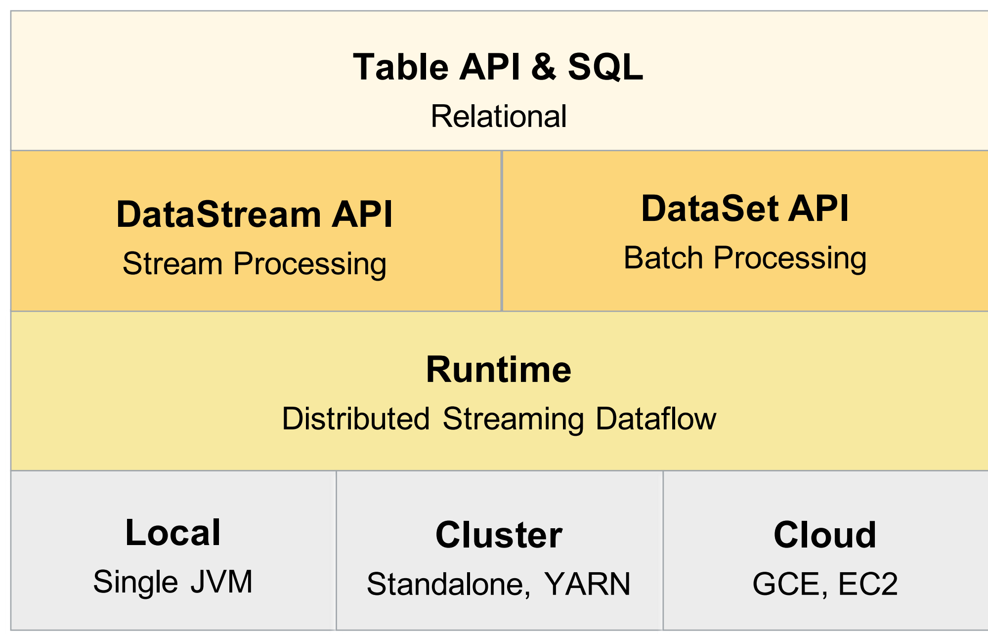
Flink Stack
