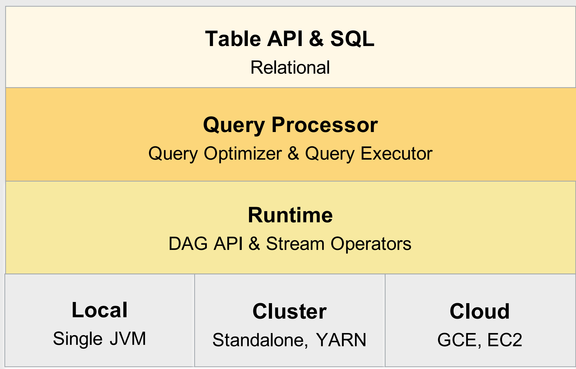
Blink Stack
