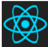
React-Native-WebRTC
